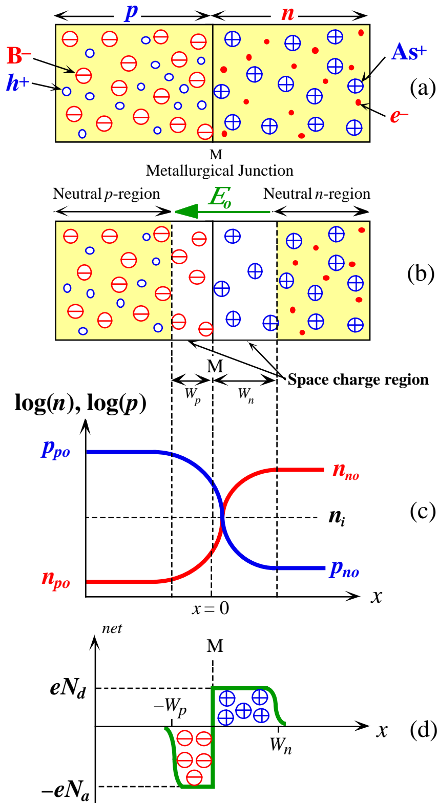
Fig. 6.1: Properties of the pn junction.
